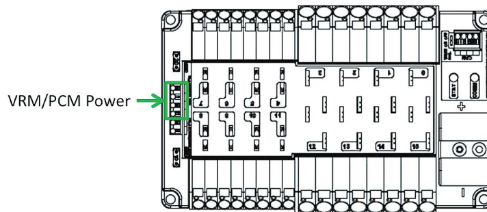
Figure 4-5: VRM/PCM Power Connection
