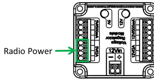
Figure 4-4: Radio Power Connection
