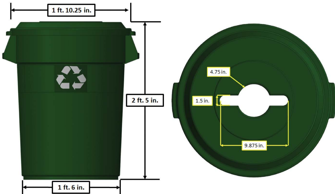
Figure 2-18: RECYCLE CONTAINER Geometry
