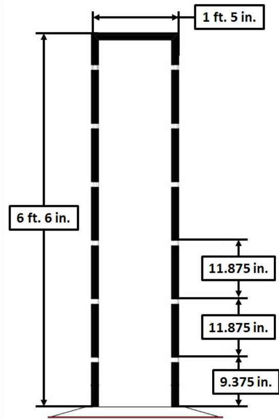
Figure 2-6: BACKSTOP Geometry
