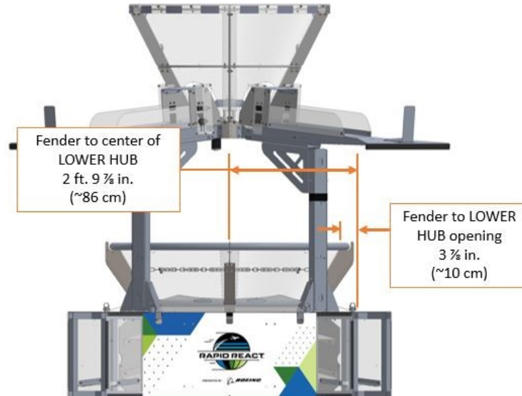
Figure 5-13 Fender geometry
