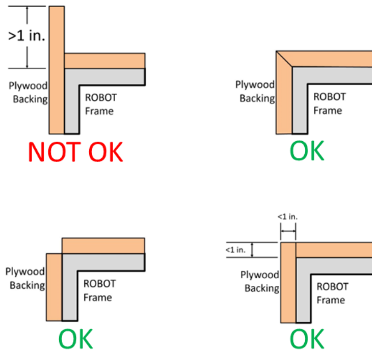
Figure 8-4 Hard parts of BUMPER corners
