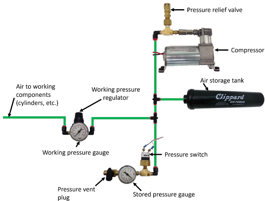
Figure 8-16 Pneumatic circuitry
