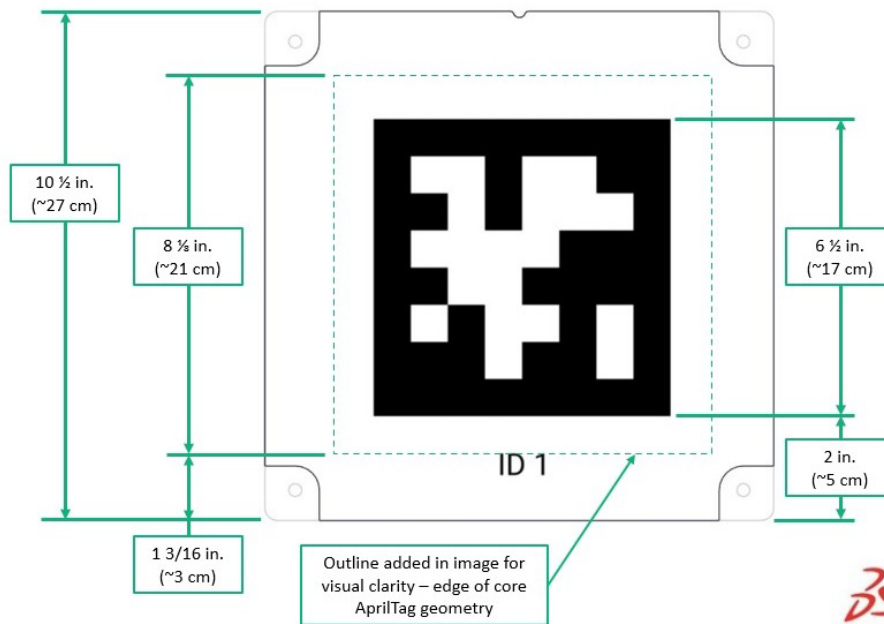
Figure 5-20 AprilTag sizing (plastic mounted, then aluminum mounted)
