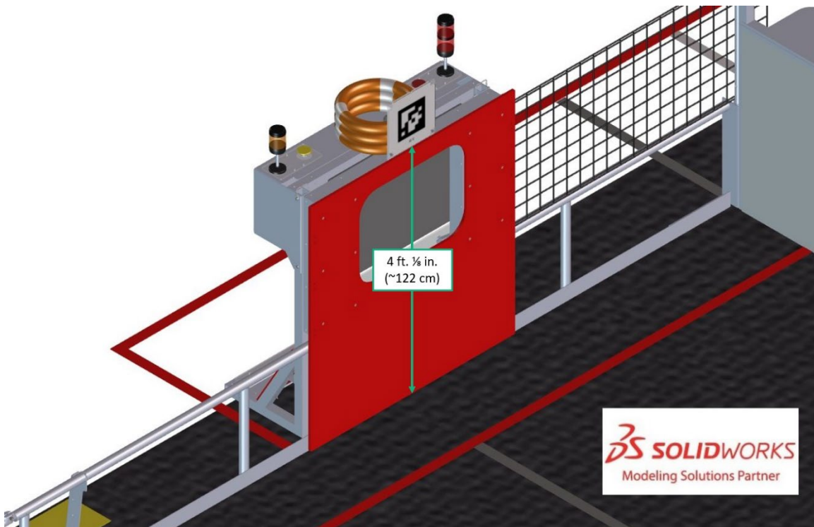
Figure 5-23 AMP AprilTag
