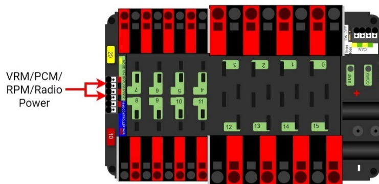
Figure 8-13 VRM, PCM, RPM, and Radio power source on a PDP
